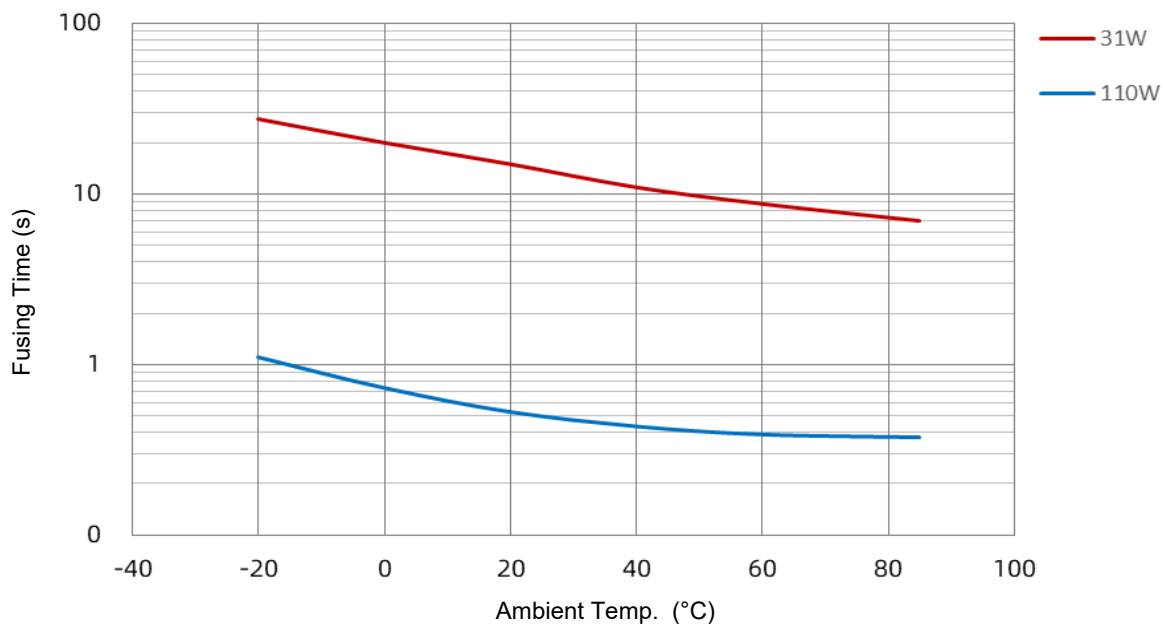
SHP 75 A Power-temp. curve
